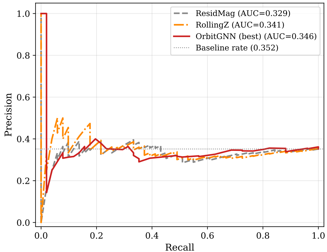
(b) Precision-Recall Curves — All Methods
