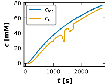
(c) reconstructed c_{int}(t) , c_p(t)
