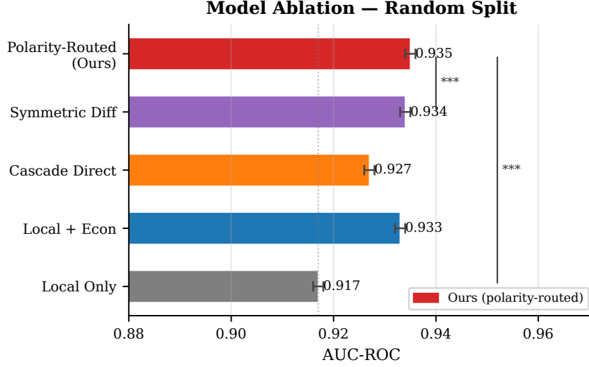
Figure 3: Random split ablation. AUC-ROC (left) and average precision (right) across model variants. Error bars show standard deviation across five seeds. Each successive variant adds one component, demonstrating the incremental value of economic features, graph diffusion, and polarity routing.
