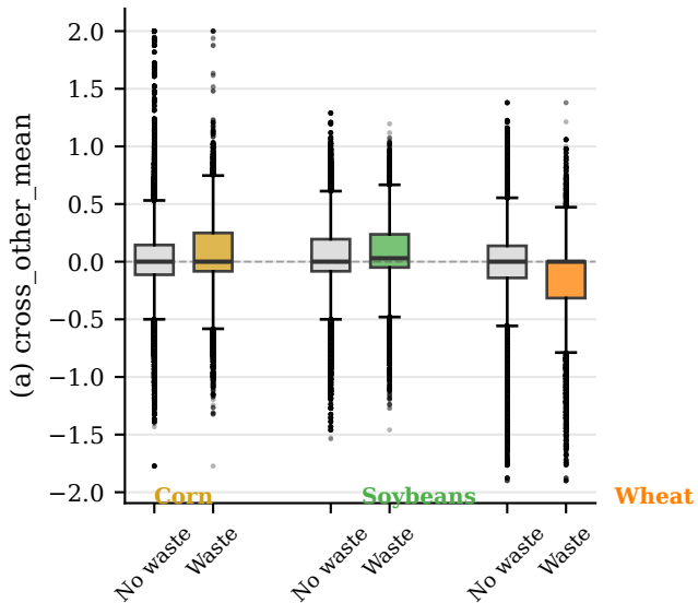
(a) cross_other_mean
