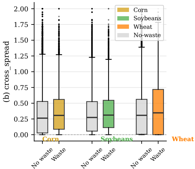
(b) cross_spread
