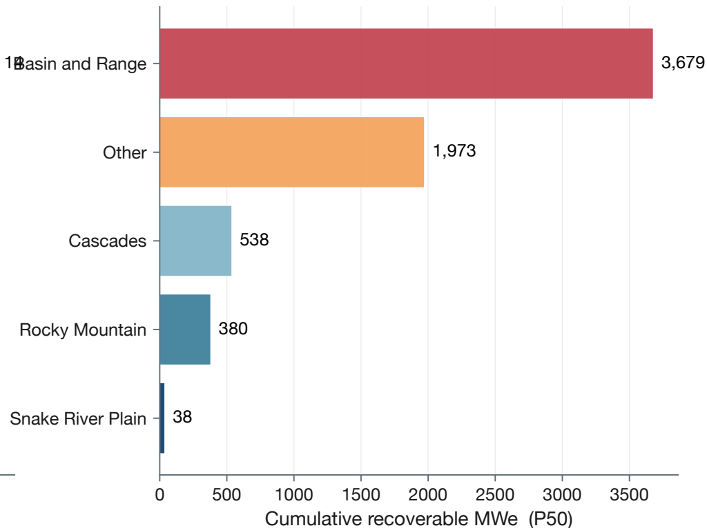
Recoverable resource per province
