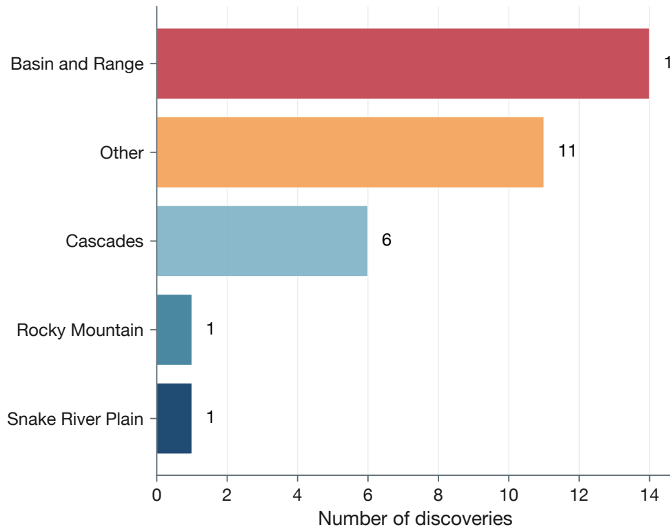
Discoveries per tectonic province
