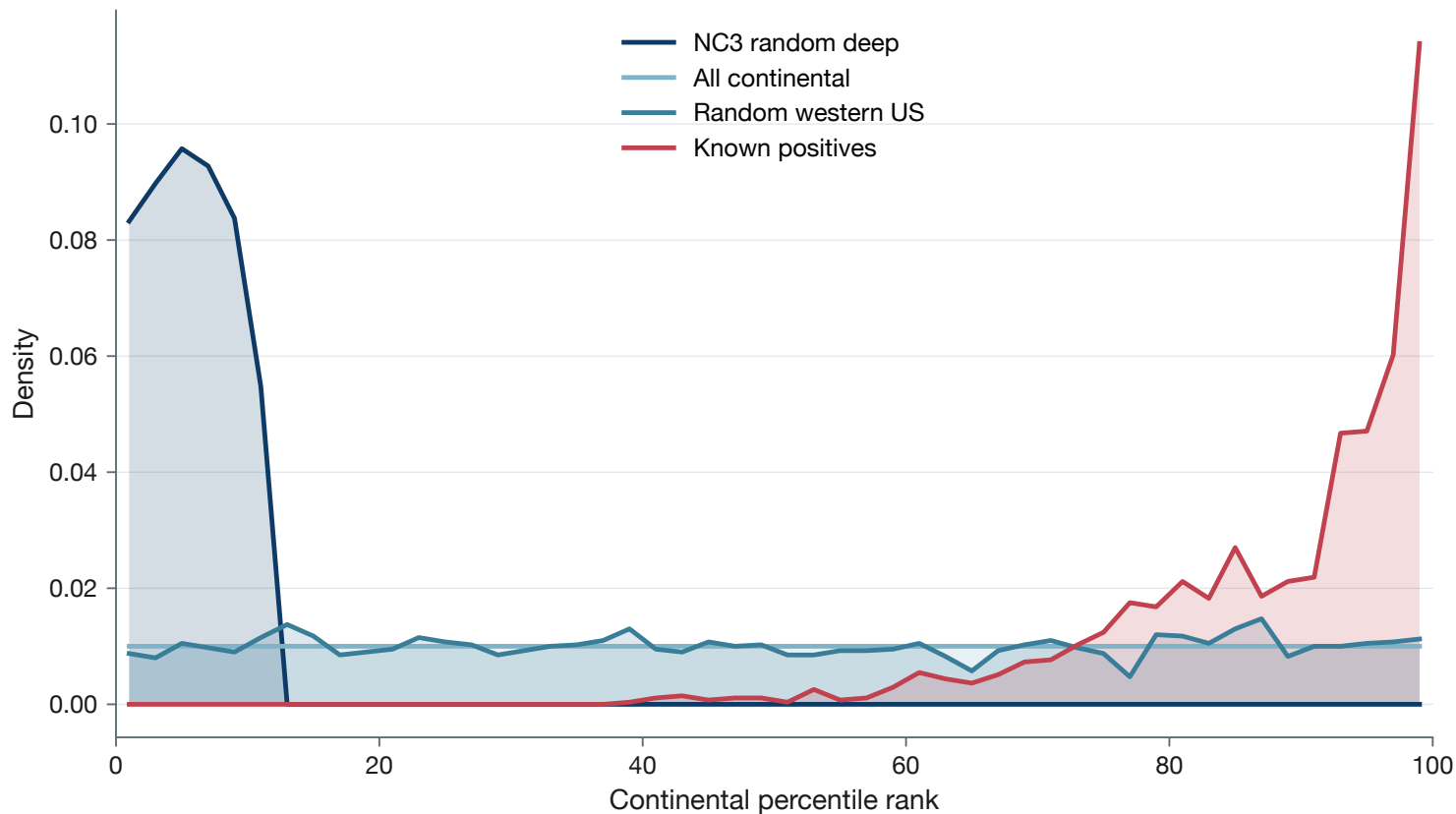
Score density by cohort
