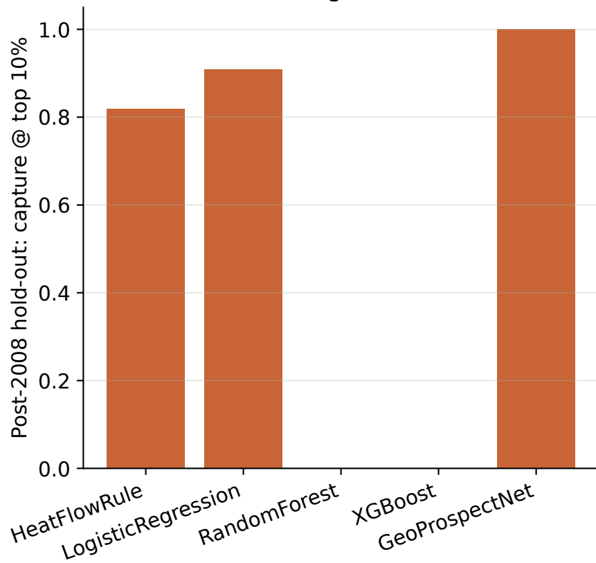
Baselines vs GeoProspectNet — generalisation gap exposed by temporal hold-out
