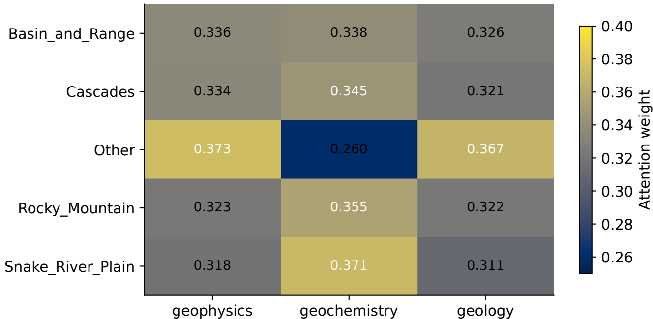
Modality attention by tectonic province
