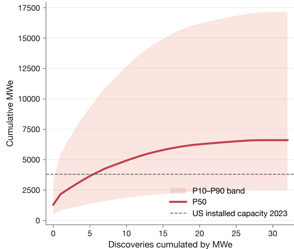
b Cumulative resource — P50 total = 6,607 MWe
