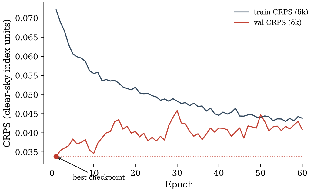
Training dynamics (closed-form mixture-CRPS objective)
