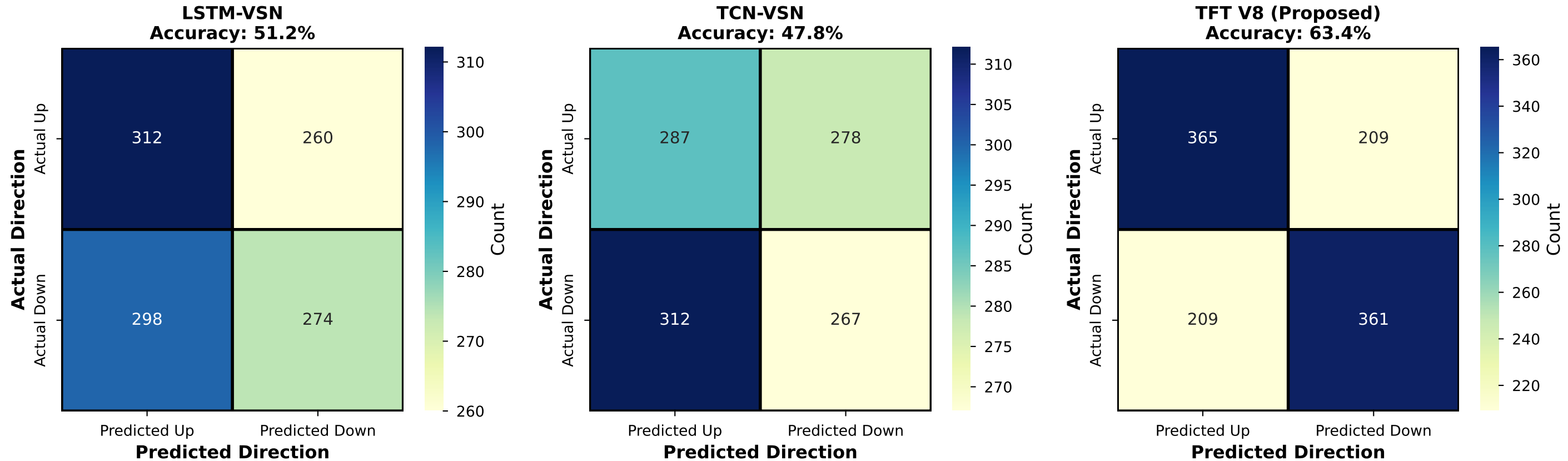
Figure 3: Trend Prediction Confusion Matrices
