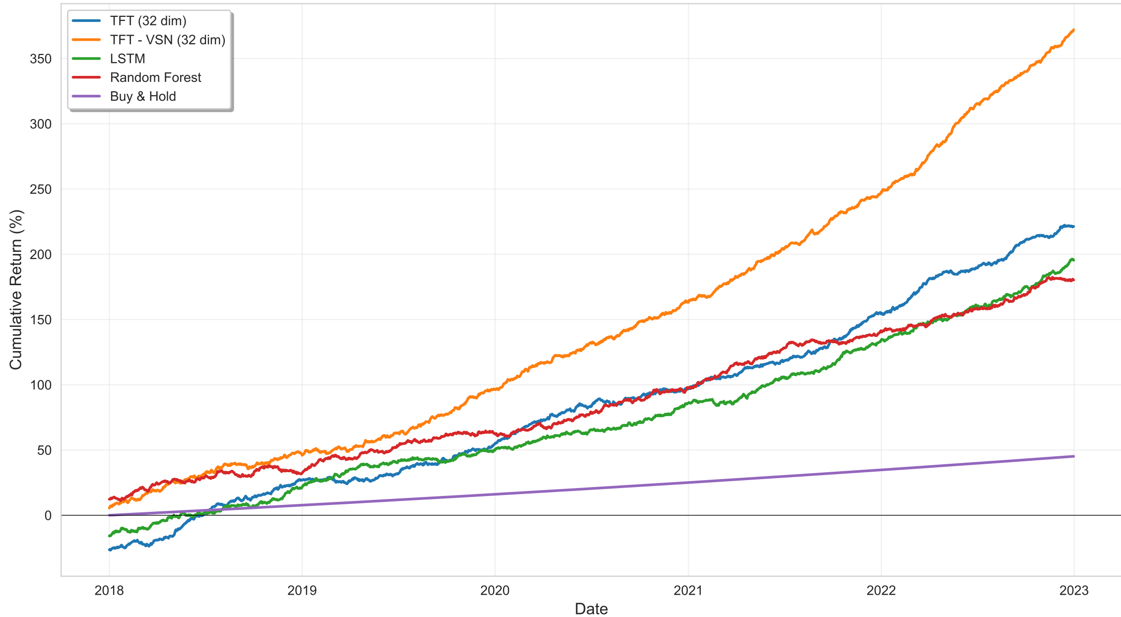
Cumulative Returns: TFT vs Baselines (2018-2022)
