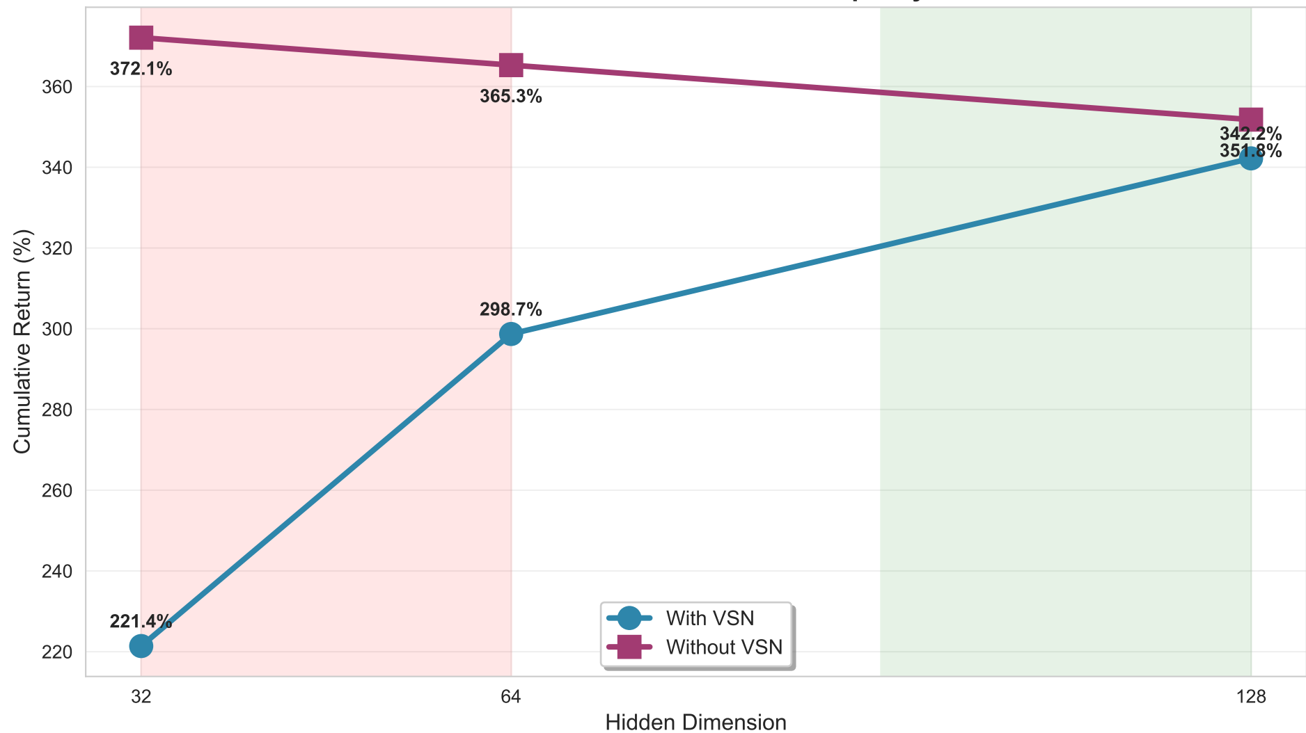
VSN Performance vs. Model Capacity
