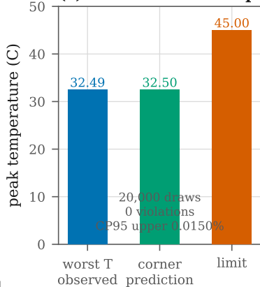
(c) 5-channel envelope, in vacuum
