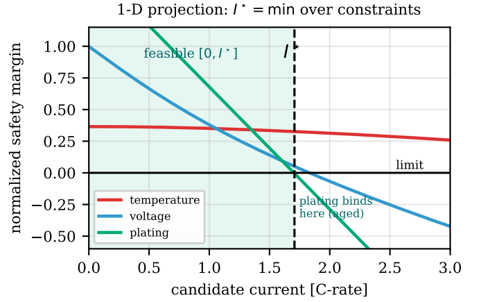
Fig. 2. The solver-free projection. Each hard constraint is monotone in the applied current, so the admissible set is a single interval and the certified cap is I^* = \min over the per-constraint roots, found by bisection with no QP.
