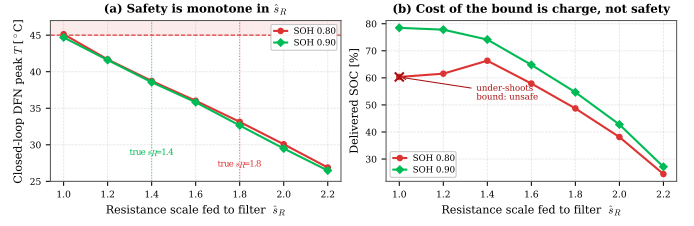
Fig. 5. Closed-loop against the DFN, safety is monotone in the resistance scale the filter is told to use (Prop. 2). (a) peak temperature falls as \hat{s}_R grows. Every value past a boundary near 1.1, well below the true aged s_R^* (dotted), is safe, so a conservative bound certifies safety without identifying s_R^* . (b) the bound’s only price is delivered charge, which is why an online estimate still earns its keep, for speed. Under-shooting the bound ( \hat{s}_R=1.0 , x) is the lone unsafe point.
