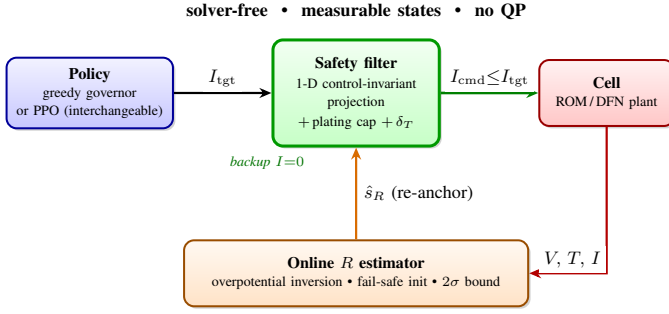
Fig. 1. Control architecture. The policy proposes a target current, the safety filter projects it to the largest value that keeps the one-step transition inside the safe set, and the online estimator re-anchors the filter to the aging cell. Only the filter carries safety.
