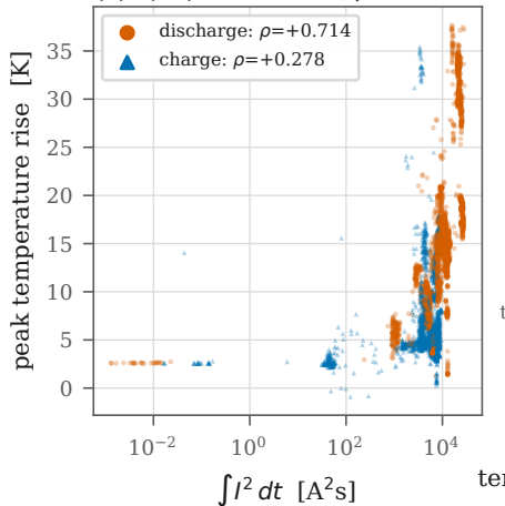
(a) 33 real cells vs the assumed bound (b) (A2) on real cells, model-free
