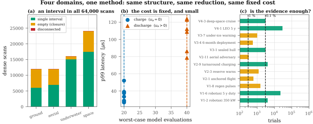
Figure 9: Four domains, one method. (a) Every dense scan returns a single interval or an empty one; none is disconnected. (b) The evaluation count is bounded at 20 on charge and 40 on discharge, and latency follows it. (c) Every headline claim clears the sample size needed to certify below 1 %.
