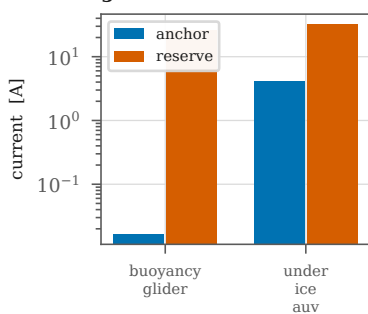
glider vs AUV: 350x load
