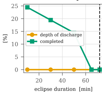
GEO comsat: eclipse season
