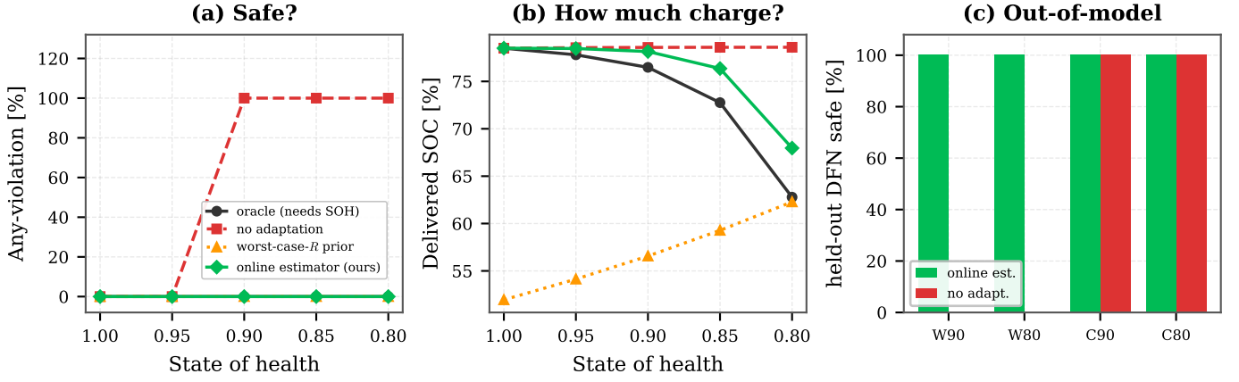
Fig. 4. Deployment across the SOH range. (a) among the filtered variants, only “no adaptation” violates, and early (100% of episodes from SOH 0.9). Oracle, worst-case- R prior, and our estimator stay at 0% in model. (b) the worst-case prior wastes charge on healthy cells while the estimator recovers the oracle’s charge. (c) held-out aged-DFN ensemble, where the estimator stays safe out of model.
