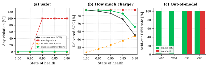
Fig. 4. Deployment across the SOH range. (a) among the filtered variants, only “no adaptation” violates, and early (100% of episodes from SOH 0.9). Oracle, worst-case- R prior, and our estimator stay at 0% in model. (b) the worst-case prior wastes charge on healthy cells while the estimator recovers the oracle’s charge. (c) held-out aged-DFN ensemble, where the estimator stays safe out of model.
