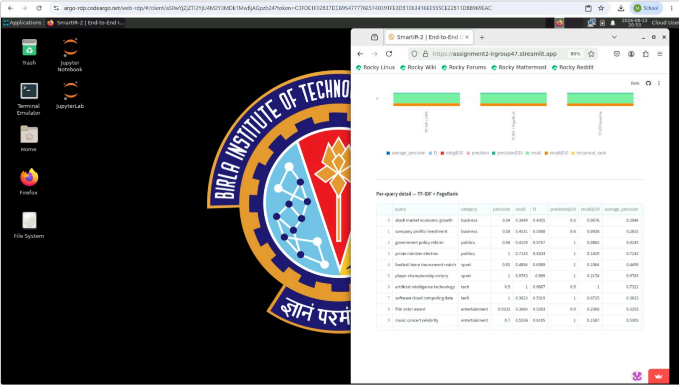
Figure 29 — Evaluation — per-query detail for TF-IDF + PageRank
