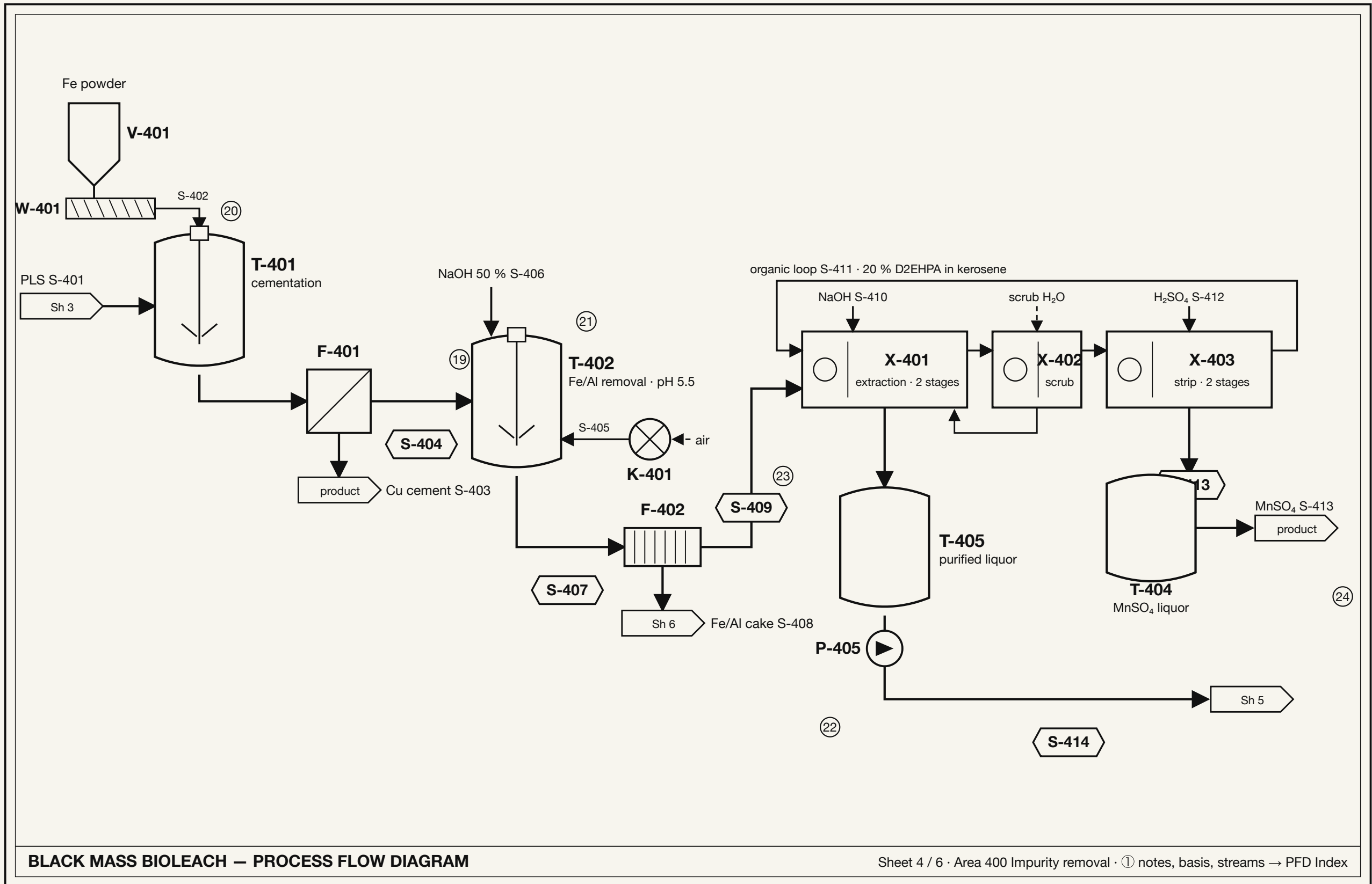
Sheet 4 — Area 400 · Impurity removal (Cu → Fe/Al → Mn)
