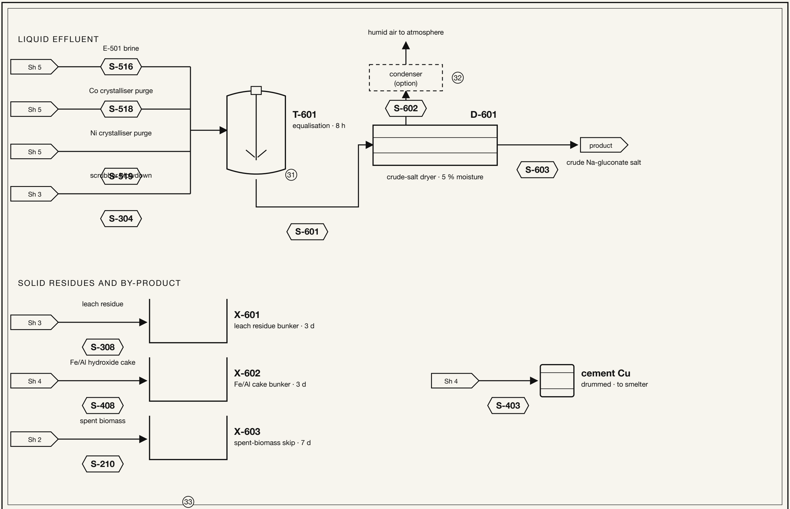
Sheet 6 — Area 600 · Effluent, by-product salt and solid residues
