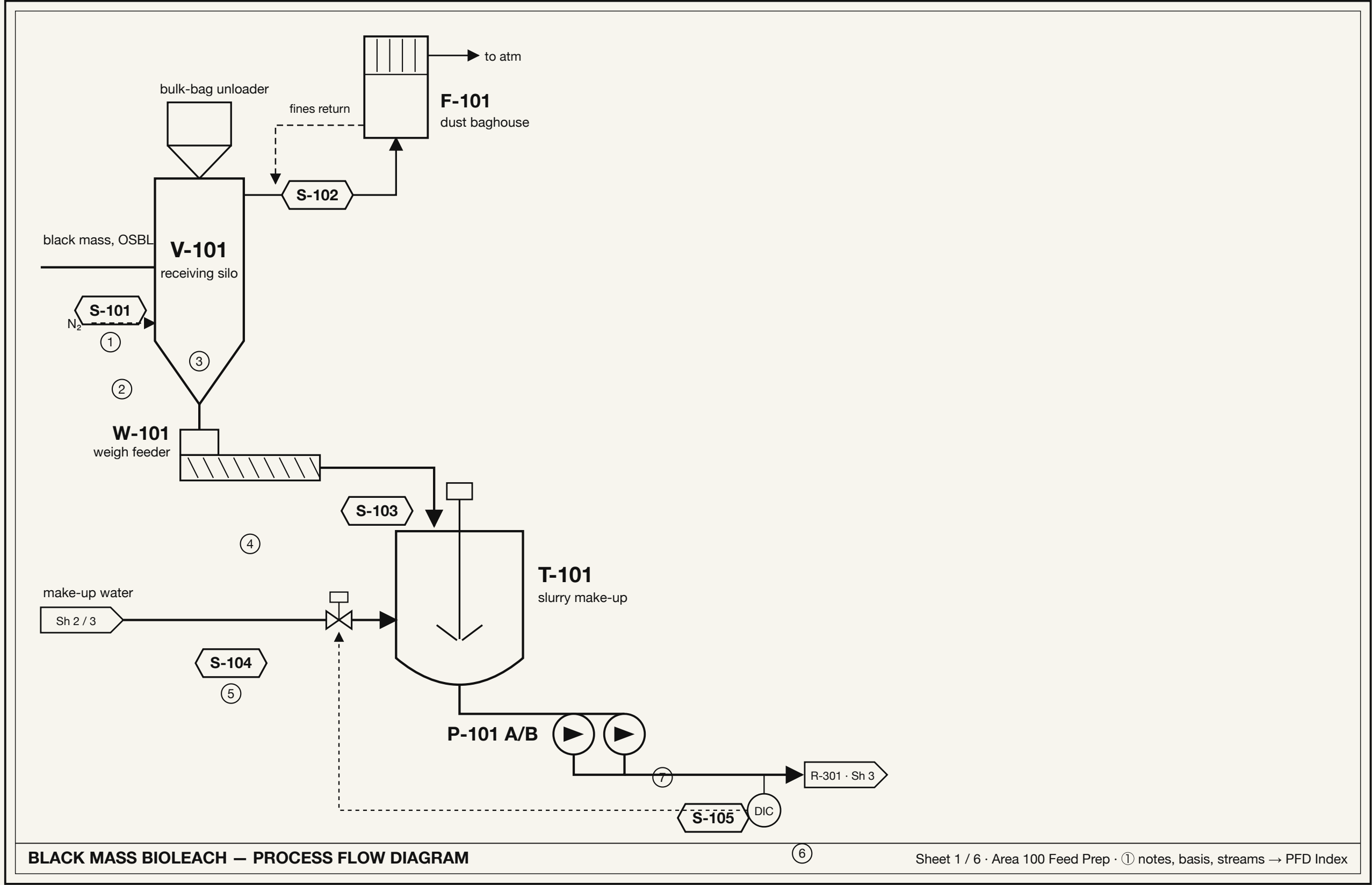
Sheet 1 — Area 100 · Feed preparation
