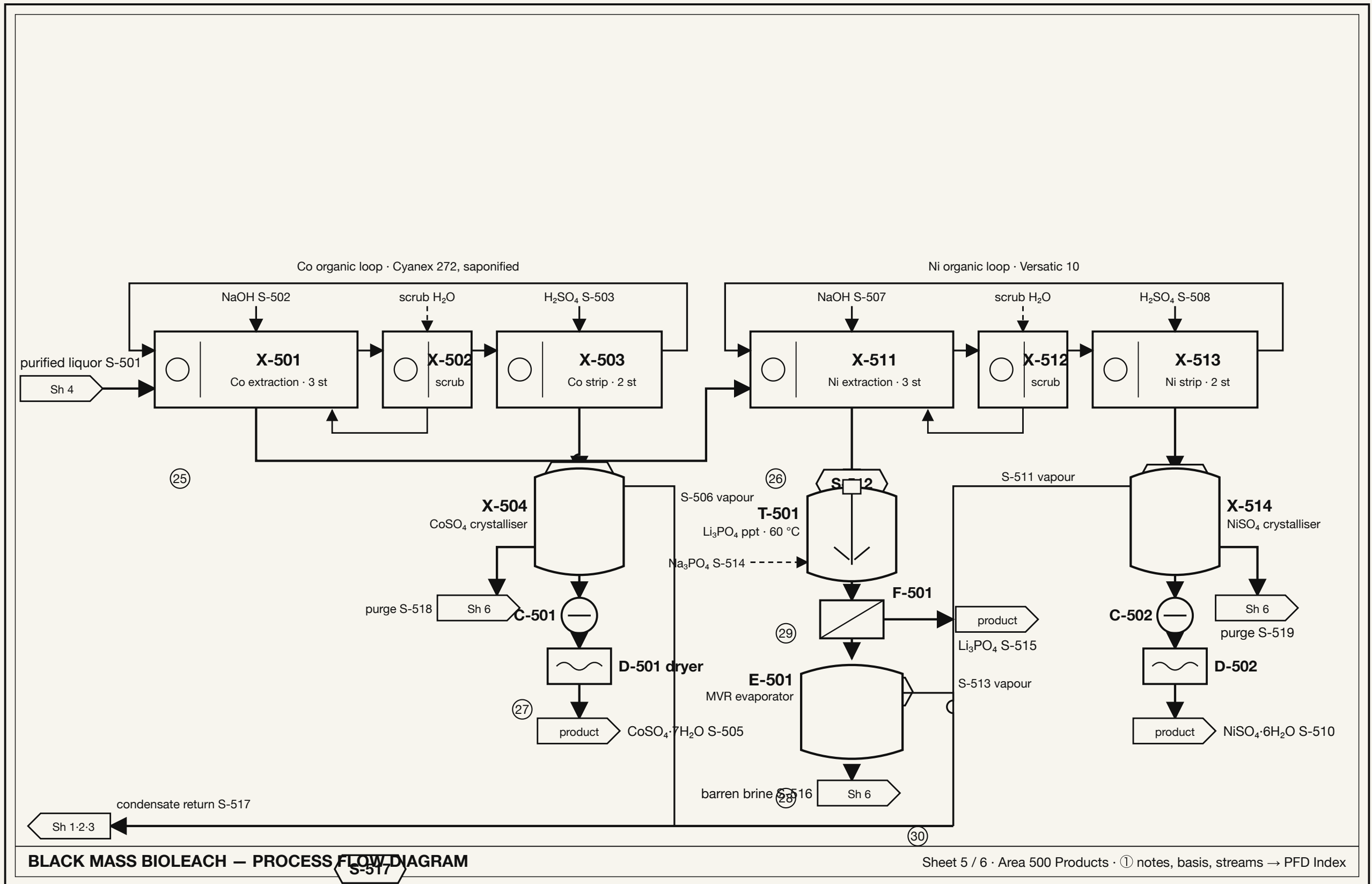
Sheet 5 — Area 500 · Products (Co SX → CoSO 4 · Ni SX → NiSO 4 · Li 3 PO 4 ) and water return
