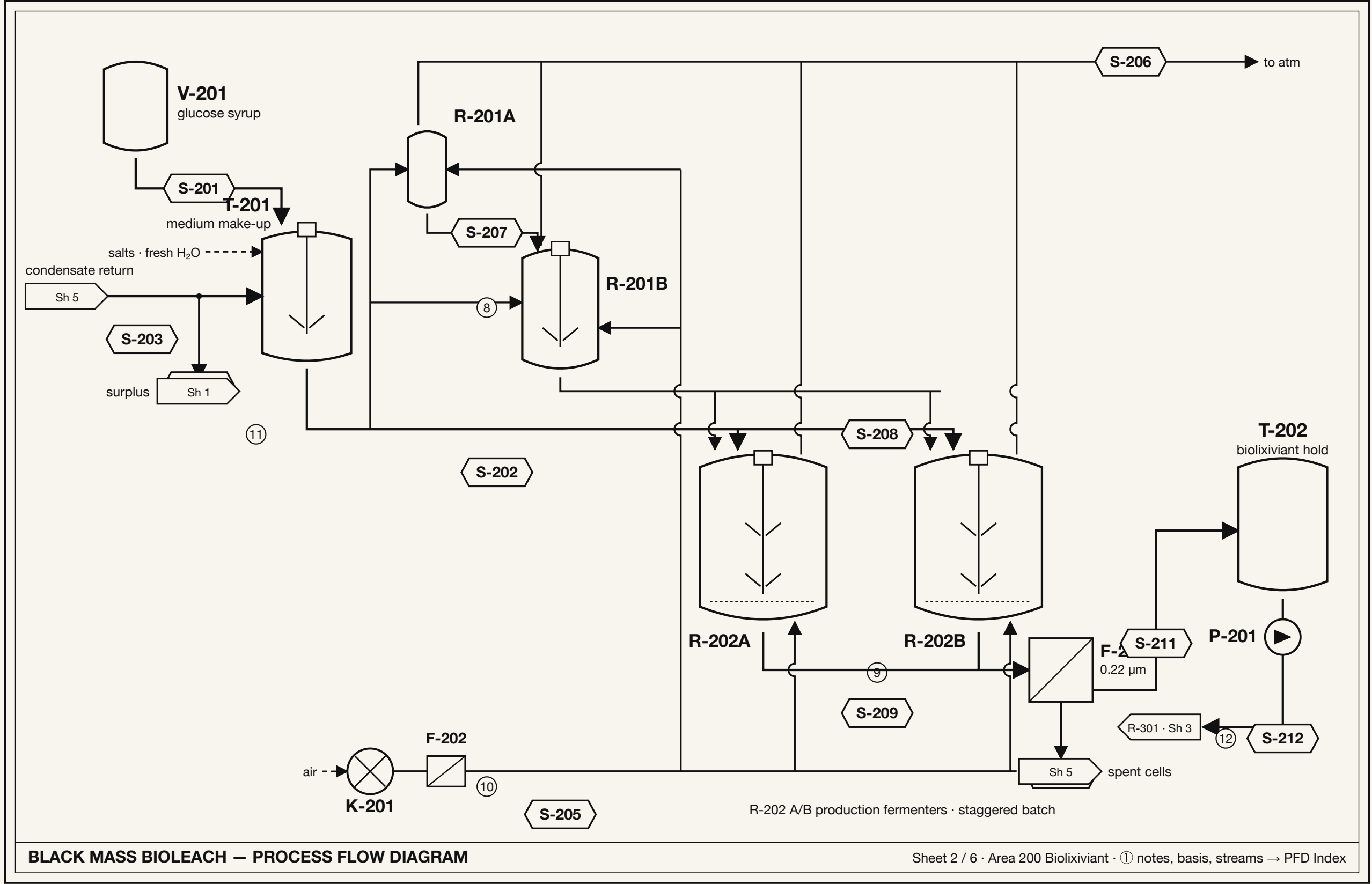
Sheet 2 — Area 200 · Biolixiviant fermentation
