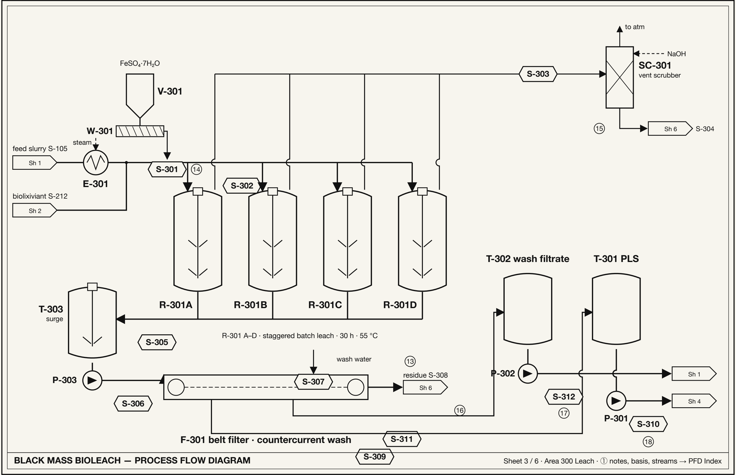
Sheet 3 — Area 300 · Batch leach and solid/liquid separation
