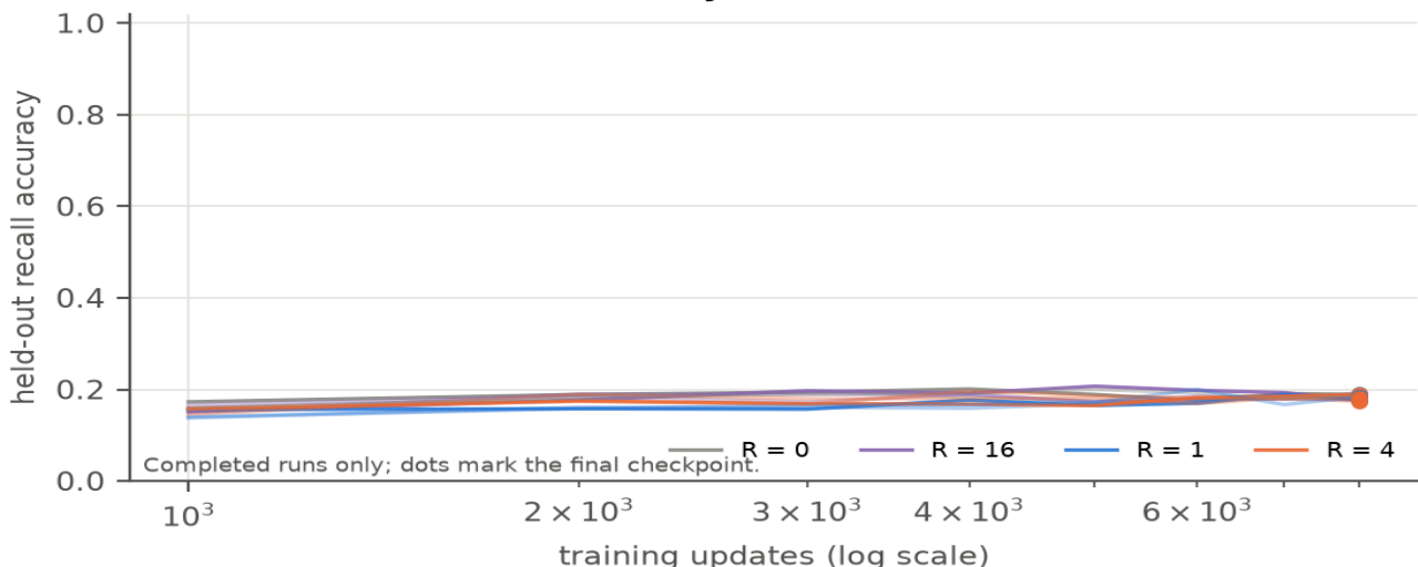
E68 · race-count ablation on synthetic recall (lines = seeds)
