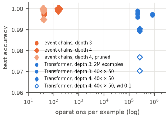
Deep order: parity at depth 3, \sim 10 \times fewer errors at depth 4 with equal data, 10^3 - 10^4 \times less work
