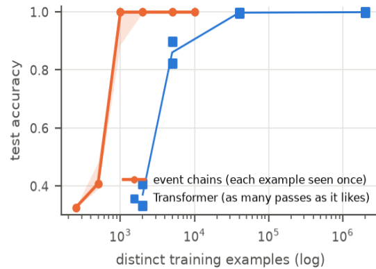
Data efficiency (depth-3 order)
