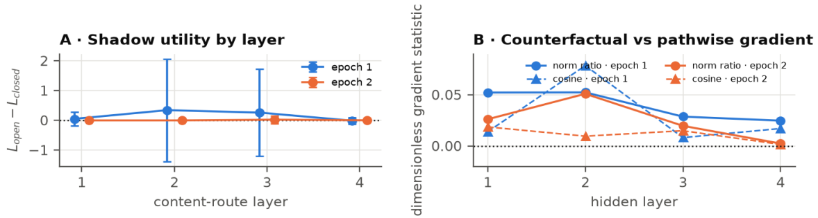
A: positive loss difference disfavors opening; bars show \pm 1 SD across sampled routes. B: norm ratio and cosine. One seed; held-out accuracy stayed near chance.
