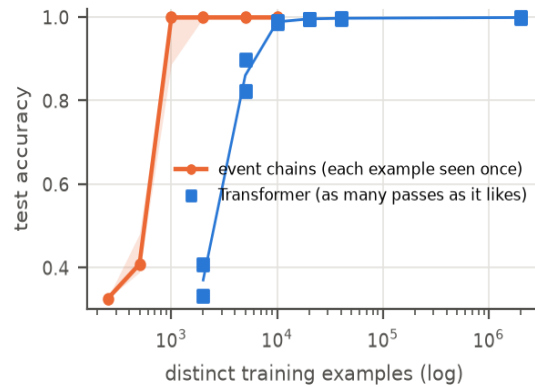
Deep order: parity at depth 3, \sim 10 \times fewer error at depth 4 with equal data, 10^3-10^4 \times less work
