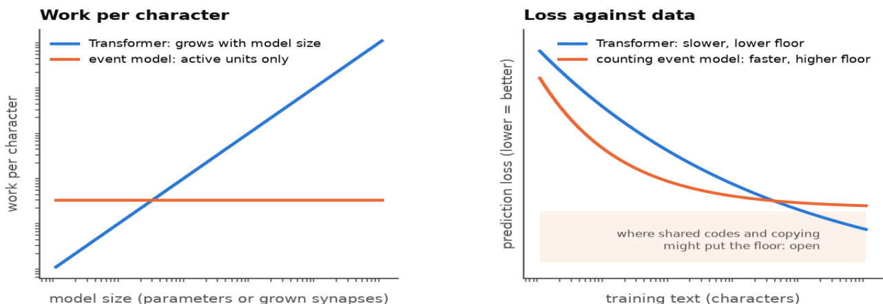
Predicted scaling (schematic, from §95; not measured)
