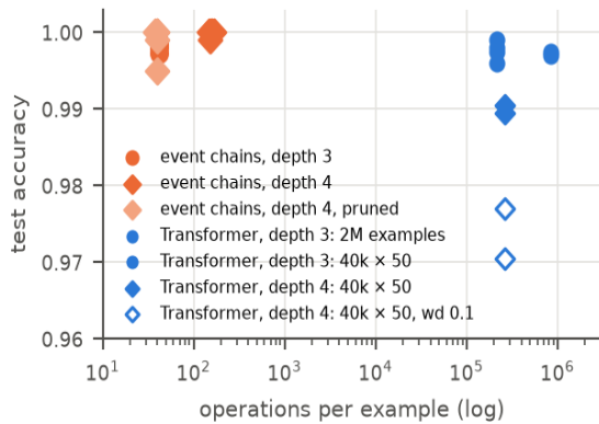
Deep order: parity at depth 3, \sim 10 \times fewer error at depth 4 with equal data, 10^3-10^4 \times less work
