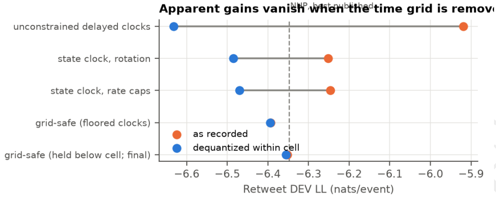
Figure 4: The recording-resolution pitfall on Retweet: apparent gains vanish under dequantization; the grid-safe model is unaffected.
