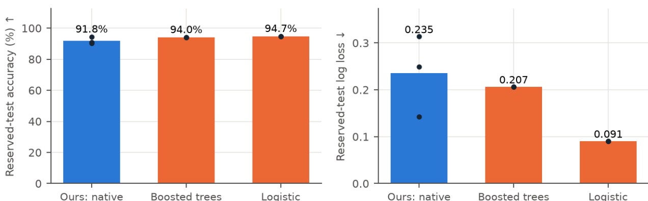
banknote reserved test
