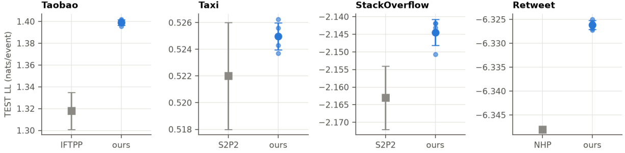
Figure 1: TEST log-likelihood: best published model (mean \pm sd over its five seeds) and ours (each seed, mean \pm sd).
