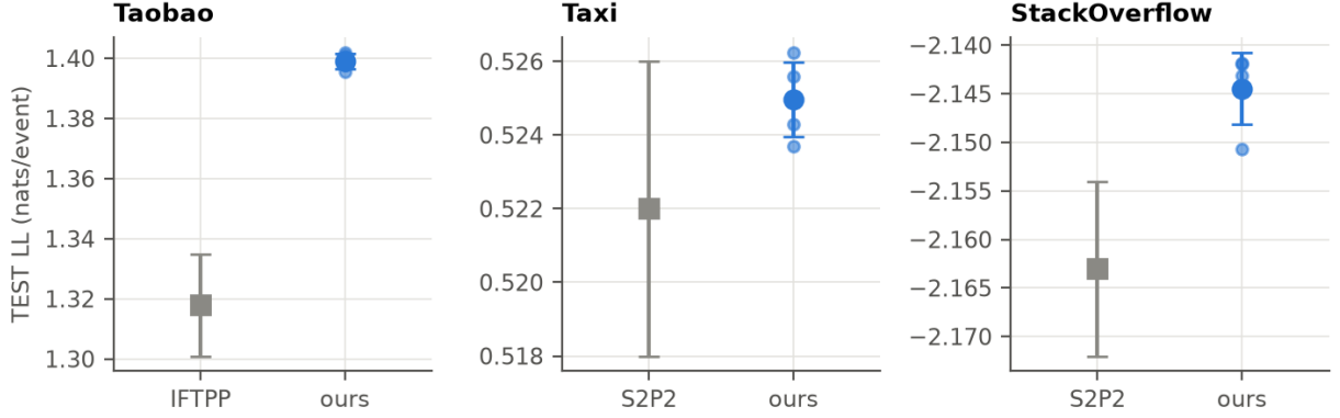
Figure 1: TEST log-likelihood: best published model (mean \pm sd over its five seeds) and ours (each seed, mean \pm sd).
