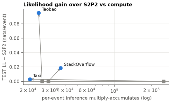
Figure 2: Gain over S2P2 against per-event compute.
