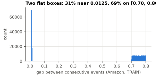
Figure 3: Amazon training gaps form two flat boxes.
