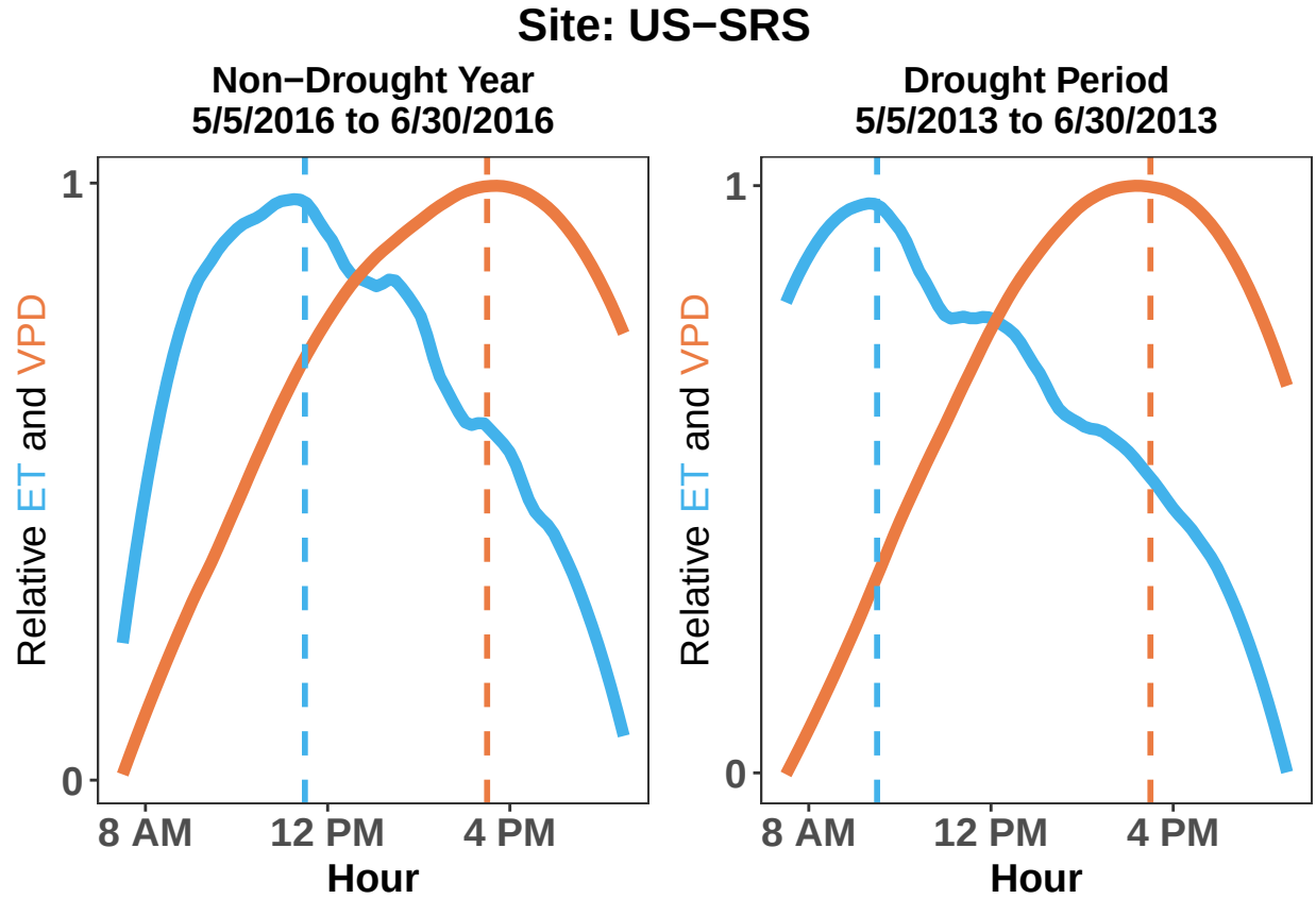
Figure 1: Illustration of the DDF using observed eddy covariance data from a woody savanna site in Arizona (Ameriflux site: US-SRS). Blue depicts ET, with VPD in red, each normalized from 0 to 1 over the day (y-axis) and averaged by hour (x-axis). Panel A shows the typical diurnal sequence during a non-drought period (May-June 2016), with peak ET occurring during midday and peak VPD in the late afternoon. Panel B shows the same time of year during a drought (May-June 2013), where peak ET shifts earlier while VPD timing remains unchanged. This shift illustrates how drought advances peak ET timing relative to peak VPD and forms the conceptual basis for the DDF
