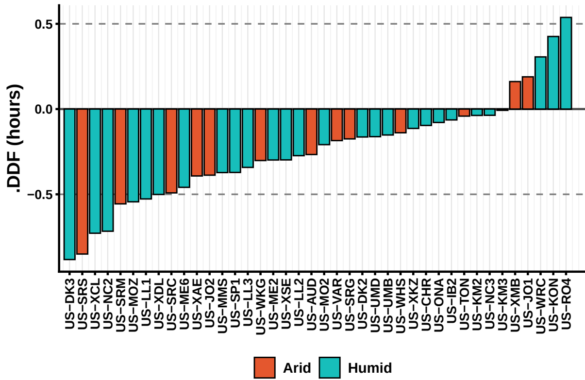
Figure 5: Site-level drought effects on mean DDF ( \Delta \text{DDF} = \text{DDF}_{\text{drought}} - \text{DDF}_{\text{ND}} ), organized by site aridity class then by magnitude of the DDF signal. Negative values indicate earlier ET peak timing during drought
