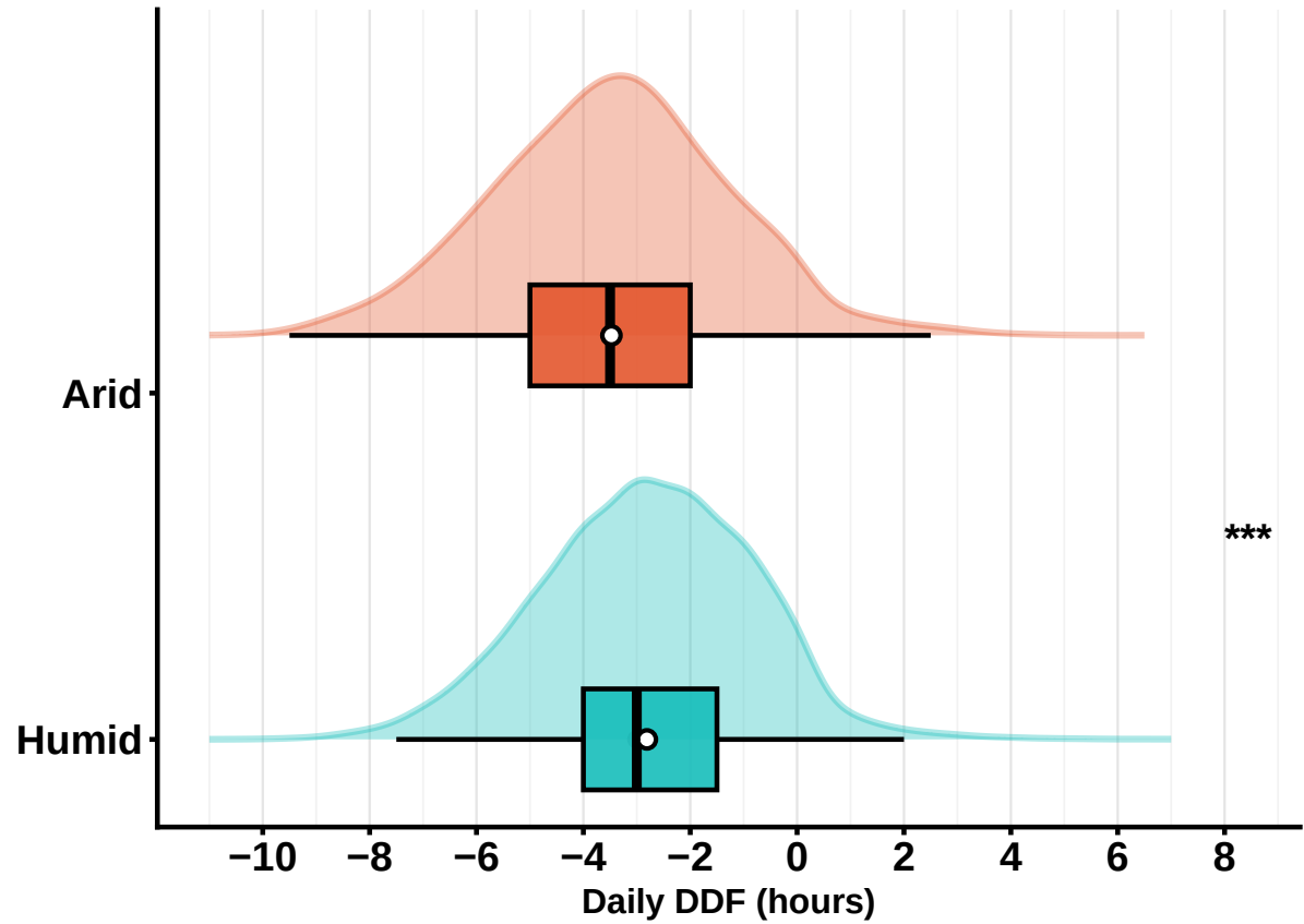
Figure 7: Comparison of DDF distributions across aridity gradients. Boxplots show medians (black horizontal lines) and means (white points); density overlays Gaussian kernel estimates (bandwidth = 0.4). Statistical significance: Welch's t-test (***) p < 0.001 . Outliers were removed for plotting purposes but not analyses
