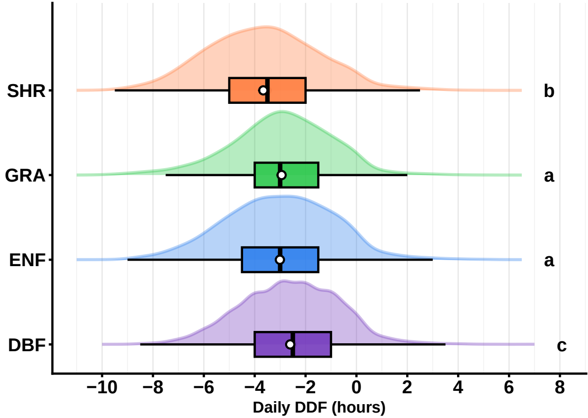
Figure 8: Comparison of DDF distributions across vegetation gradients. Boxplots show medians (black horizontal lines) and means (white points); density overlays Gaussian kernel estimates (bandwidth = 0.4). Statistical significance: Tukey HSD post-hoc comparisons (letters denote statistically significant groups). Outliers were removed for plotting purposes but not analyses
