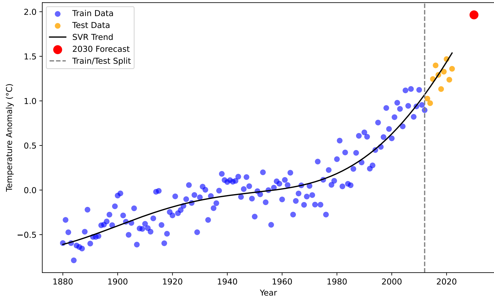
Global Temperature Anomaly Forecast (Figure 5)
