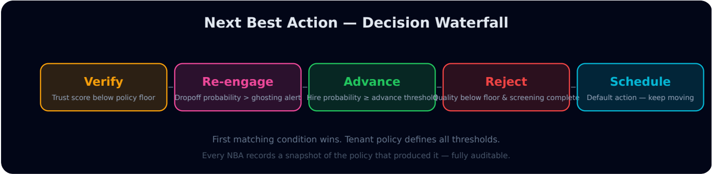
Figure 3 — Next Best Action waterfall (first match wins)
