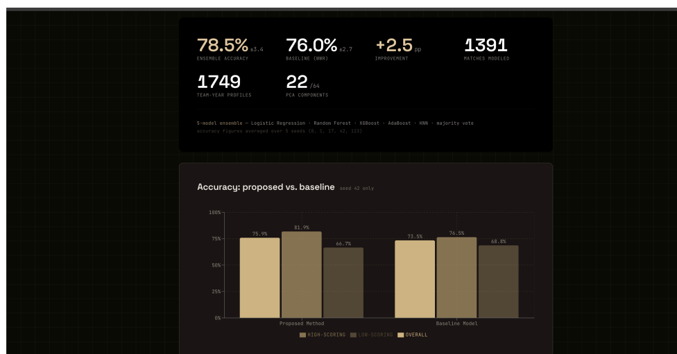
Figure 13: The top of the evaluation-results dashboard: headline stat tiles (ensemble accuracy, baseline, improvement, matches modeled) and the accuracy-vs-baseline chart.
