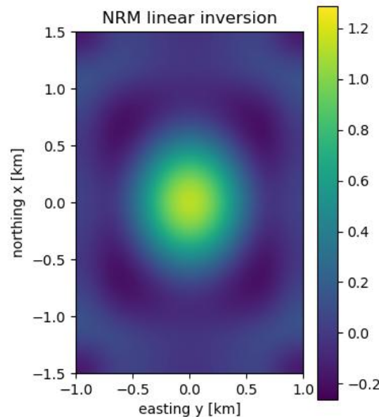
Magnetic test 2:
