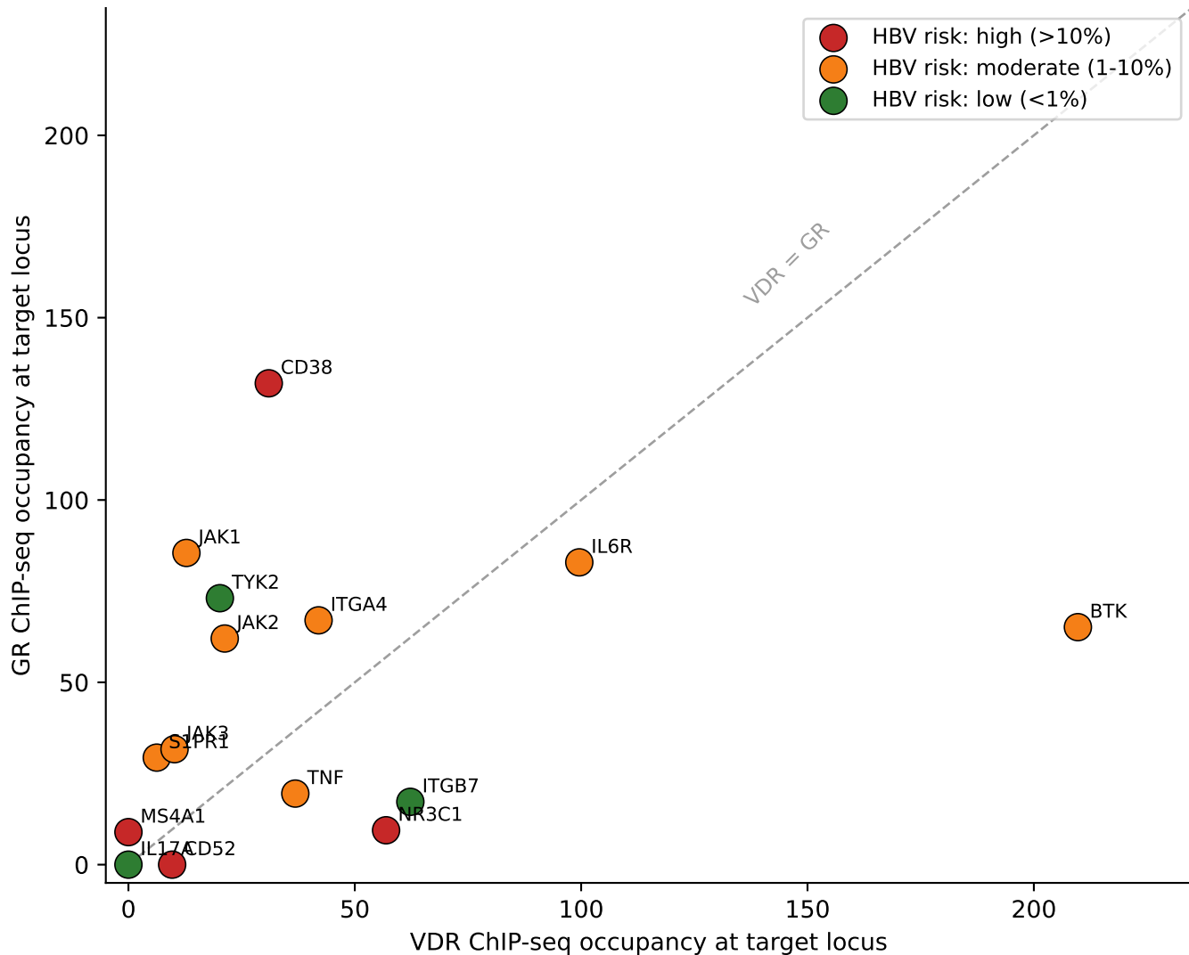
HBV-reactivation risk vs VDR/GR occupancy (no association: Spearman rho=-0.08, p=0.77; Kruskal-Wallis p=0.27)
