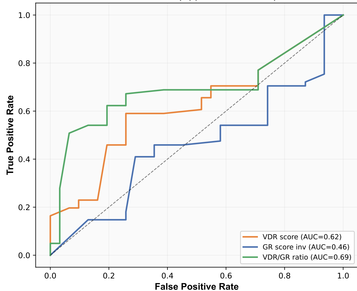
ROC Curves (Approved vs Failed)
