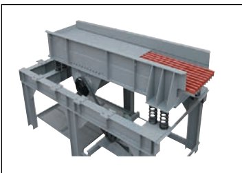
❖ 진동피더 Vibrating Feeder
