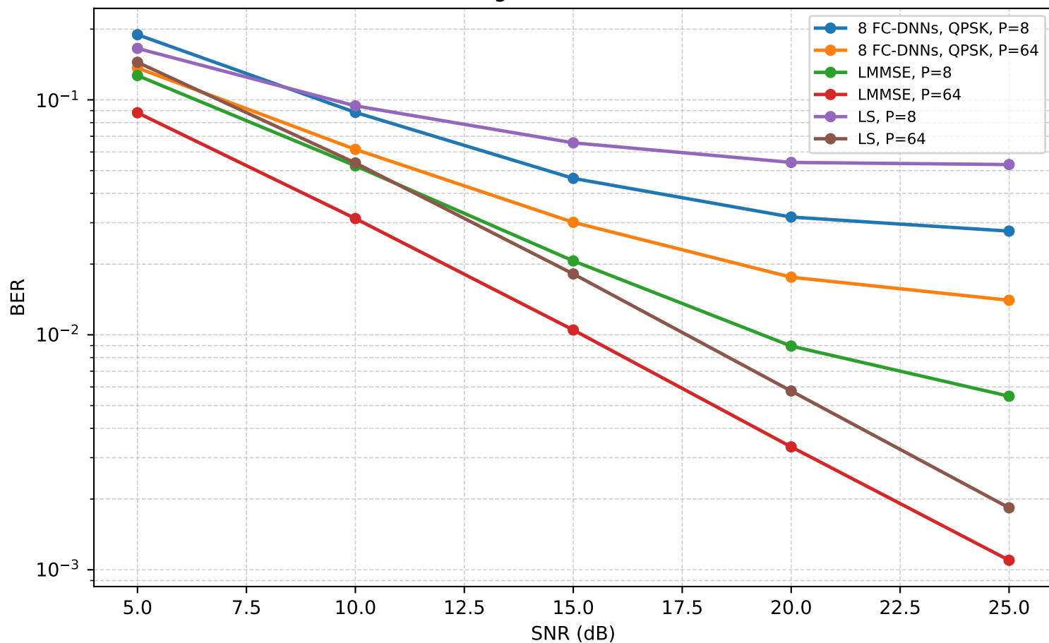
OFDM Signal Detection BER - b
