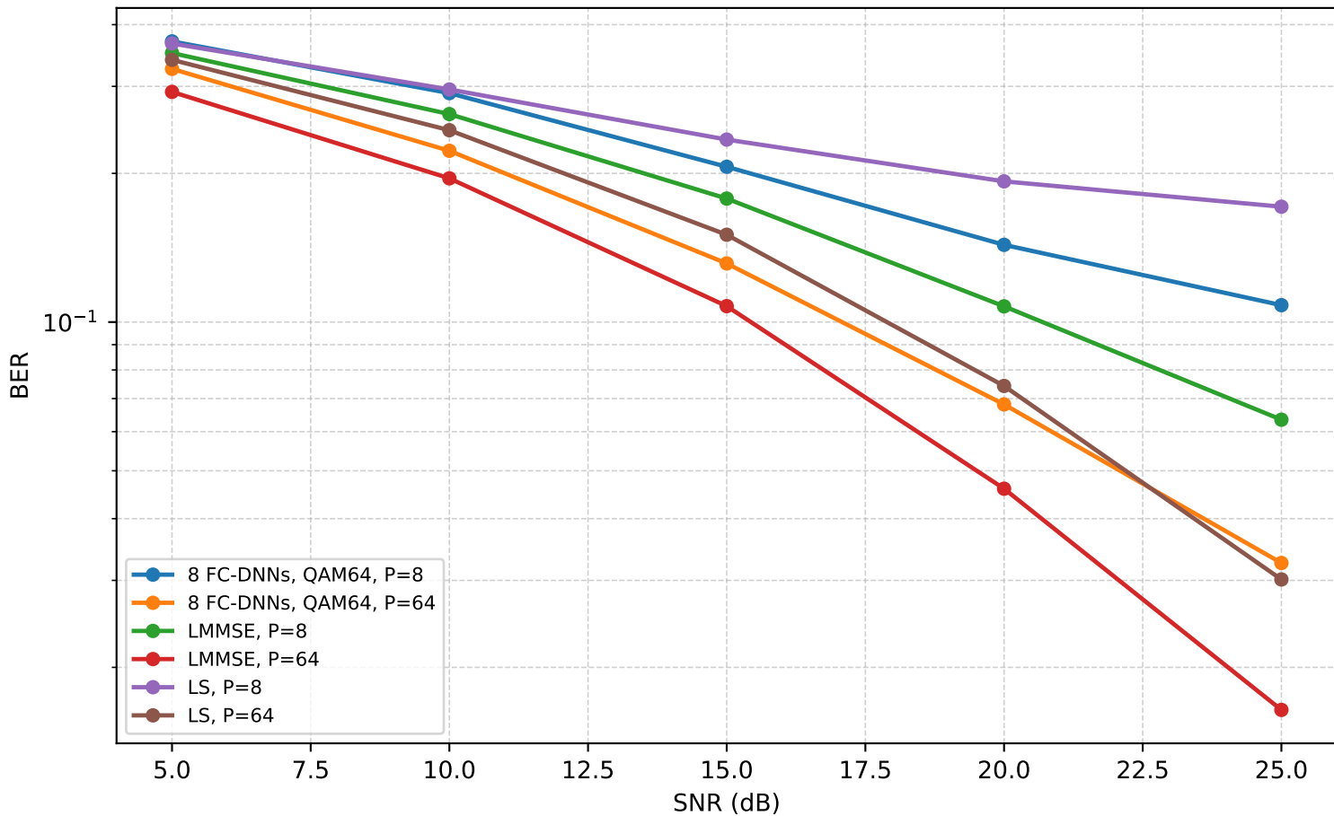
OFDM Signal Detection BER - c
