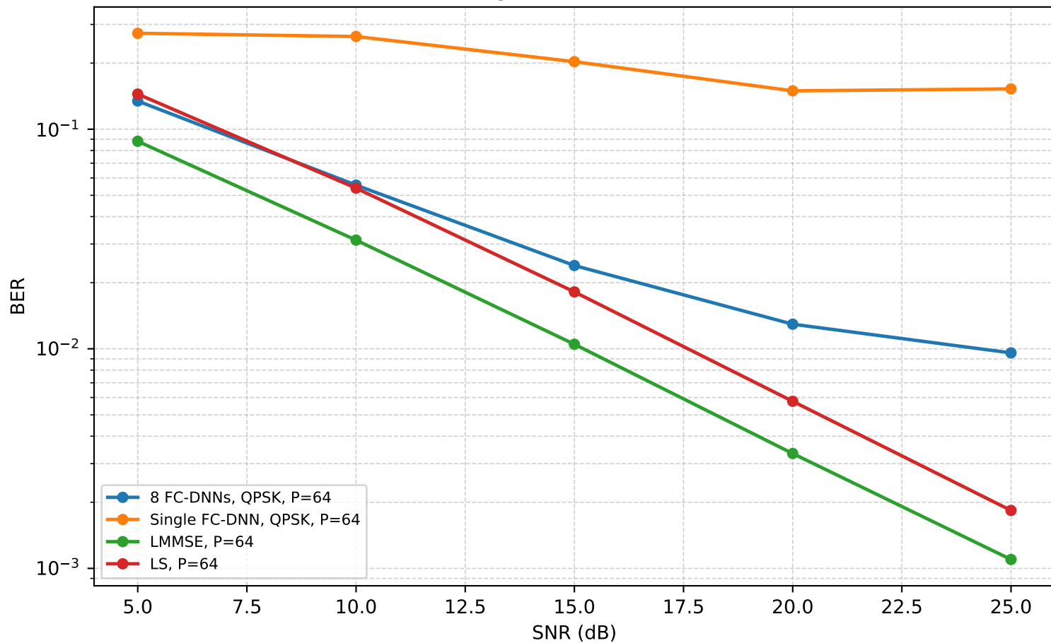
OFDM Signal Detection BER - d
