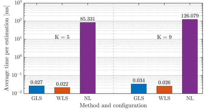
Fig. 9. Computation latency of the NLS, GLS, and WLS estimators for K = 5 and K = 9 .
