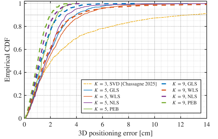
Fig. 7. Empirical CDF of the 3D positioning error for K \in \{3, 5, 9\} ( M=1,000 Monte Carlo trials, 1,792 testbed positions). Solid lines: K=5 ; dashed lines: K=9 ; dash-dotted: K=3 SVD baseline [22]. Each estimator uses its respective GA-optimized orientation set.
