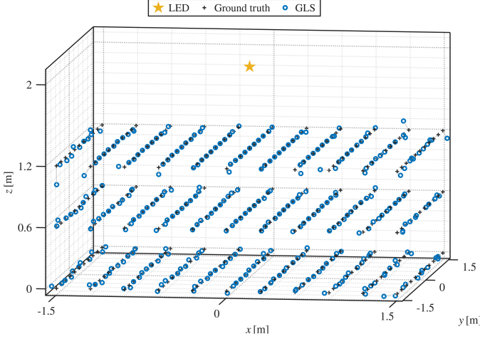
Fig. 8. 3D position estimates produced by GLS ( K=5 ) at receiver heights z \in \{0, 0.6, 1.2\} \text{ m} in the 3 \times 3 \times 2 \text{ m}^3 room. The LED transmitter is at the ceiling ( z = 2 \text{ m} ); segments connect each reference position to the corresponding estimate.
