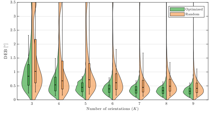
Fig. 2. Distribution of the DEB [°] across all receiver locations in the 3 \times 3 \times 2 m 3 testbed for K \in \{3, \dots, 9\} . Green: GA-optimized orientation set; orange: randomly selected set. Box-and-whisker plots summarize the sample distribution; shaded profiles depict the estimated PDF. The GA-optimized sets consistently achieve lower DEB and tighter distributions across all K .
