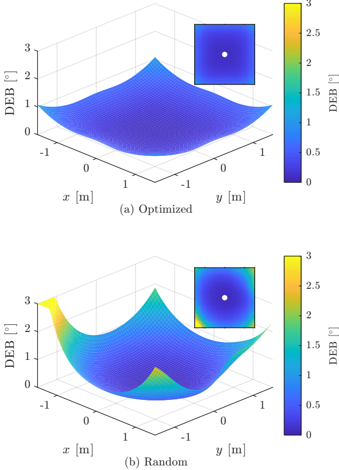
Fig. 3. Spatial distribution of the DEB across the 3 \times 3 \text{ m}^2 floor at z = 0.8 \text{ m} for K = 5 orientations. (a) GA-optimized set; (b) randomly selected set. The colour scale is shared and clipped at 3^\circ .
