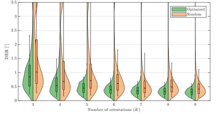
Fig. 2. Distribution of the DEB [\circ] across all receiver locations in the 3 \times 3 \times 2 m 3 testbed for K \in \{3, \dots, 9\} , with \Phi_{1/2} = 45^\circ . Green: GA-optimized orientation set; orange: 50 independently drawn random orientation sets per K . Box-and-whisker plots summarize the sample distribution; shaded profiles depict the estimated PDF. The GA-optimized sets consistently achieve lower DEB and tighter distributions across all K .
