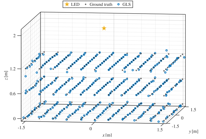
Fig. 9. 3D position estimates produced by GLS ( K = 5 ) at receiver heights z \in \{0, 0.6, 1.2\} m in the 3 \times 3 \times 2 \text{ m}^3 room. The LED transmitter is at the ceiling ( z = 2 m); segments connect each reference position to the corresponding estimate.
