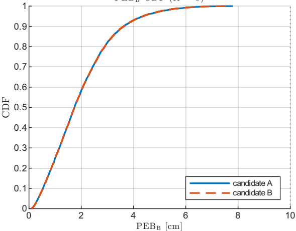
PEB B CDF ( K = 9 )
