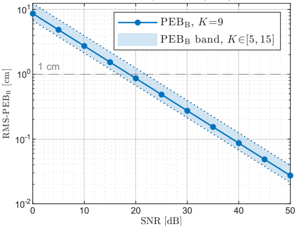
Broadcast PEB vs SNR ( \Phi_{1/2}=45^\circ , \mathbf{n}_r=[0,0,1]^T , DEB-opt.)
