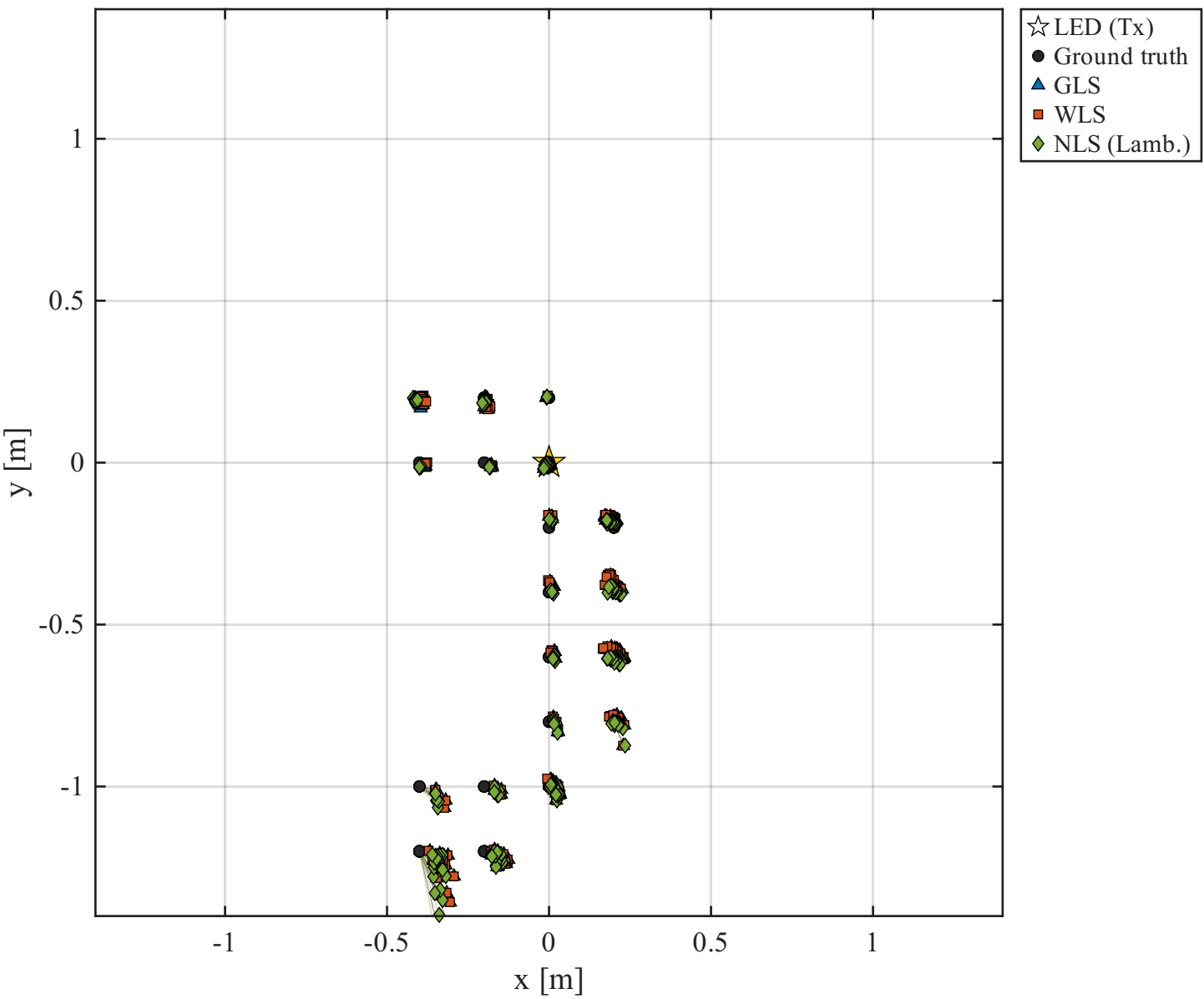
Top-view localization (X-Y) tilt PD | K_{id}=[1\ 2\ 3\ 4\ 5\ 6\ 7\ 8\ 9] | m=3.13 | NLS:Lamb
