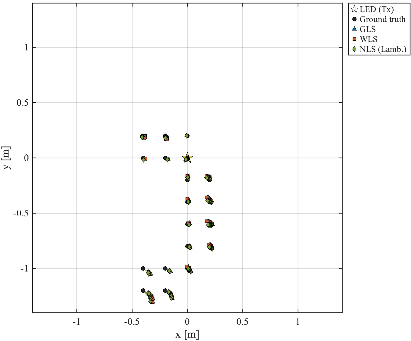
Top-view localization (X-Y) vertical PD | K_{id}=[1\ 2\ 3\ 4\ 5\ 6\ 7\ 8\ 9] | m=3.13 | NLS:Lamb
