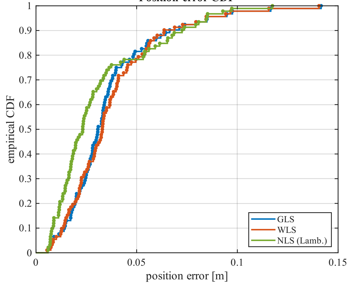
Position-error CDF
