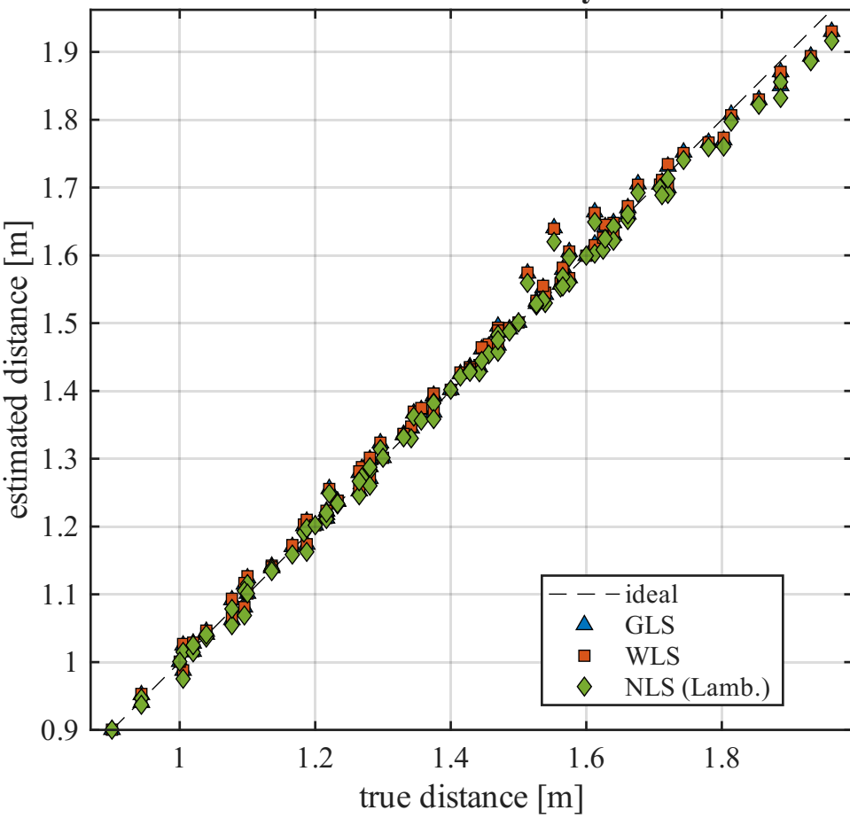
Distance recovery
