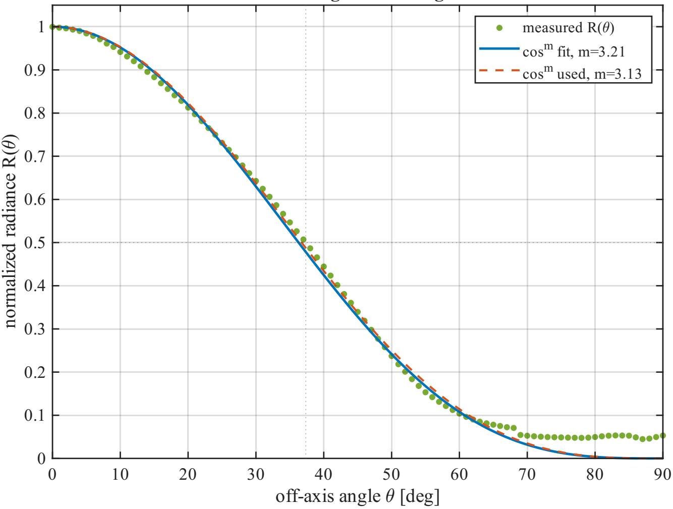
LED radiation profile (sub0 axis sweep) half-angle = 37.4 deg
