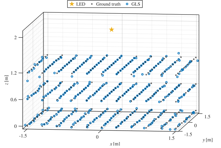
Fig. 9. 3D position estimates produced by GLS ( K=5 ) at receiver heights z \in \{0, 0.6, 1.2\} m in the 3 \times 3 \times 2 m 3 room. The LED transmitter is at the ceiling ( z = 2 m); segments connect each reference position to the corresponding estimate.
