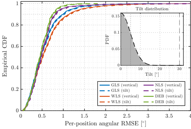
Fig. 6. Empirical CDF of the per-position angular RMSE for K=5 orientations ( M=1,000 noise trials, 1,792 positions). Solid curves: vertical receiver ( \mathbf{n}_r=[0, 0, 1]^T ); dashed curves: random receiver tilt ( N_{\text{tilt}}=100 realizations per position). Each estimator uses its GA-optimized orientation set. Inset: truncated half-normal tilt distribution ( \sigma=5^\circ , \theta_{\max}=30^\circ ). The near-perfect overlap between solid and dashed curves confirms that receiver-orientation variations have negligible impact on direction-finding accuracy (Section VI-C).
