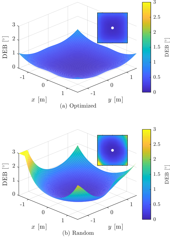
Fig. 3. Spatial distribution of the DEB across the 3 \times 3 \text{ m}^2 floor at z = 0.8 \text{ m} for K = 5 orientations. (a) GA-optimized set; (b) a single random set with tilt-azimuth pairs drawn uniformly from the GA search range. The colour scale is shared and clipped at 3^\circ .
