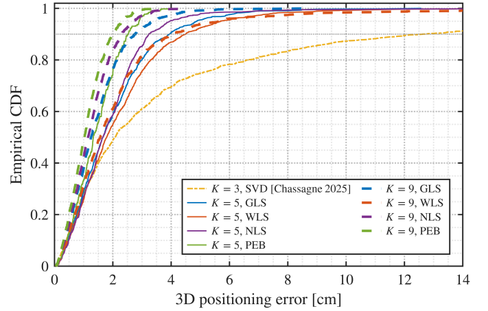
Fig. 8. Empirical CDF of the 3D positioning error for K \in \{3, 5, 9\} ( M=1,000 Monte Carlo trials, 1,792 testbed positions). Solid lines: K=5 ; dashed lines: K=9 ; dash-dotted: K=3 SVD baseline [22]. Each estimator uses its respective GA-optimized orientation set.
