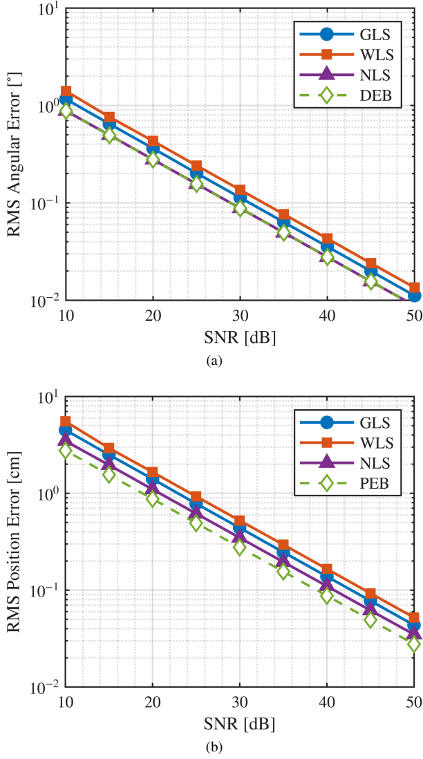
Fig. 10. Realized estimator performance vs. SNR for K=5 ( M=1,000 Monte Carlo trials, 1,792 testbed positions). (a) RMS angular error (direction finding): NLS coincides with the DEB; GLS and WLS remain at constant factors \approx 1.3\times and \approx 1.6\times . (b) RMS 3D positioning error: all estimators track the PEB with the same constant-factor offsets. All curves follow the 1/\sqrt{\text{SNR}} slope.
