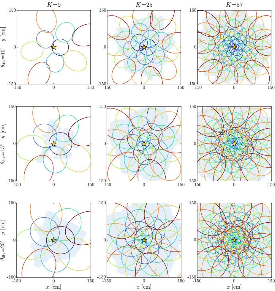
Per-beam footprints (SNR \geq 10 dB) @ z = 0.8 m — sunflower codebook
