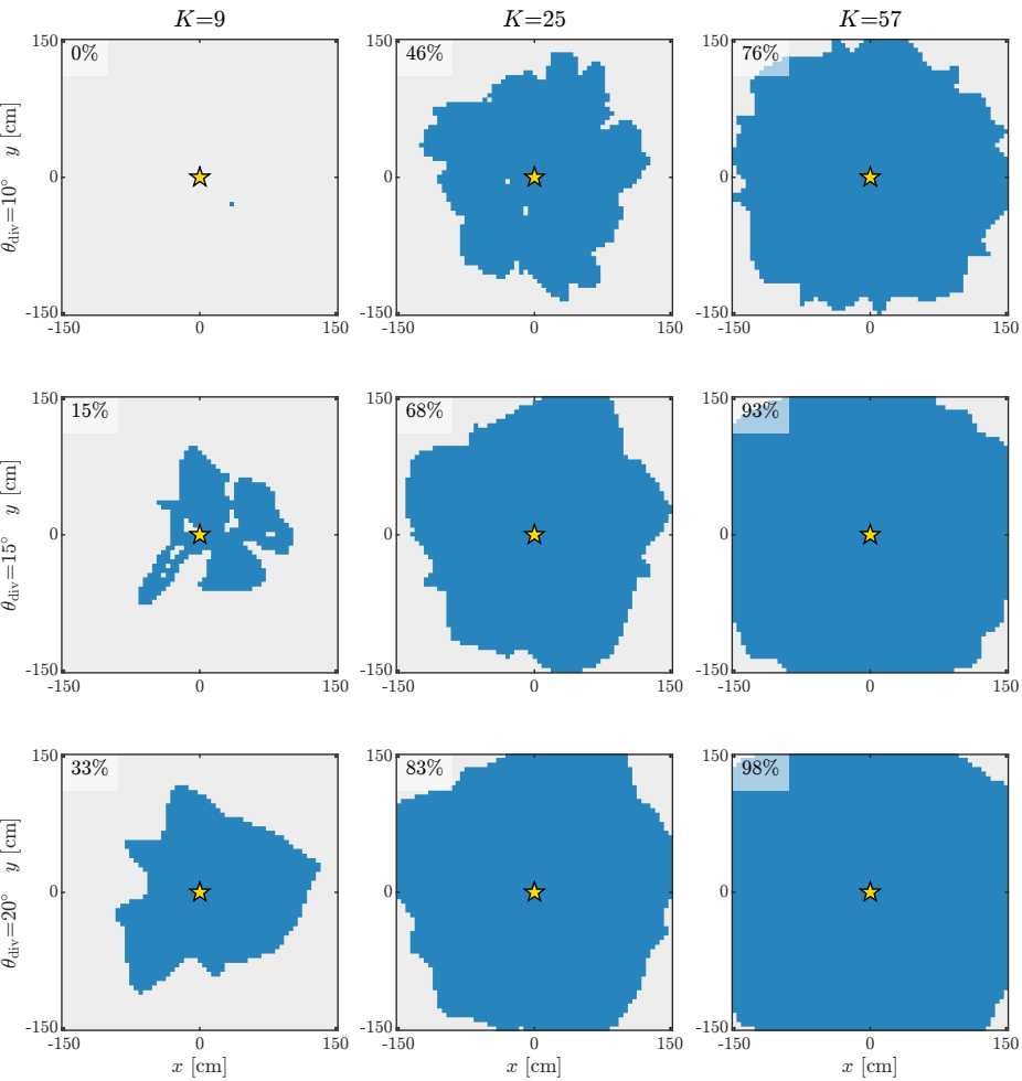
Localization coverage @ z = 0.8 m – sunflower codebook (blue = covered)
